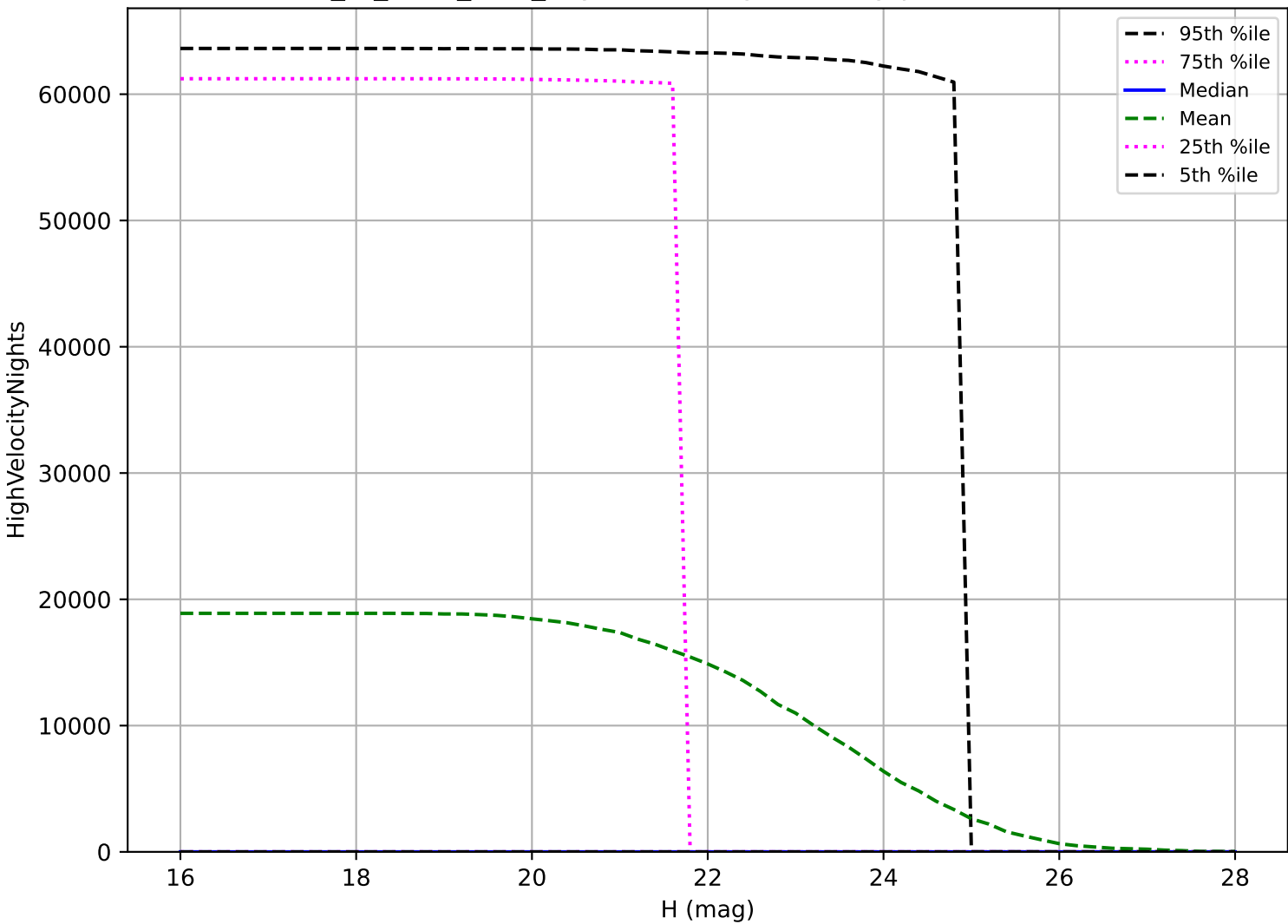
extra_ss_neo3_v3.4_10yrs: NEO High velocity pair detection loss
