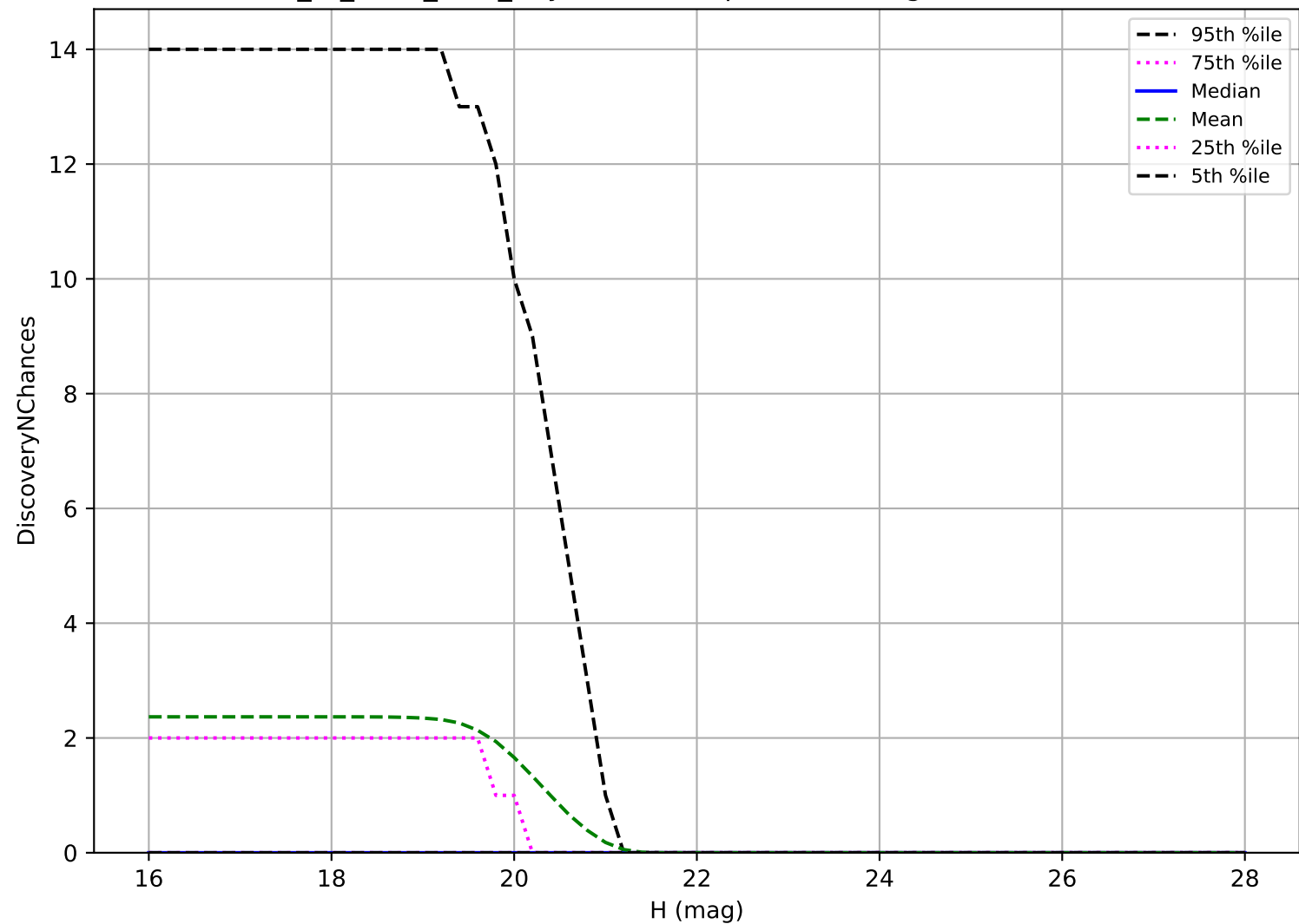
extra_ss_neo3_v3.4_10yrs: Vatira 3 pairs in 15 nights detection loss
