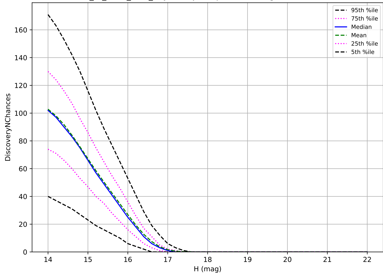
extra_ss_neo3_v3.4_10yrs: Trojan 3 pairs in 15 nights detection loss
