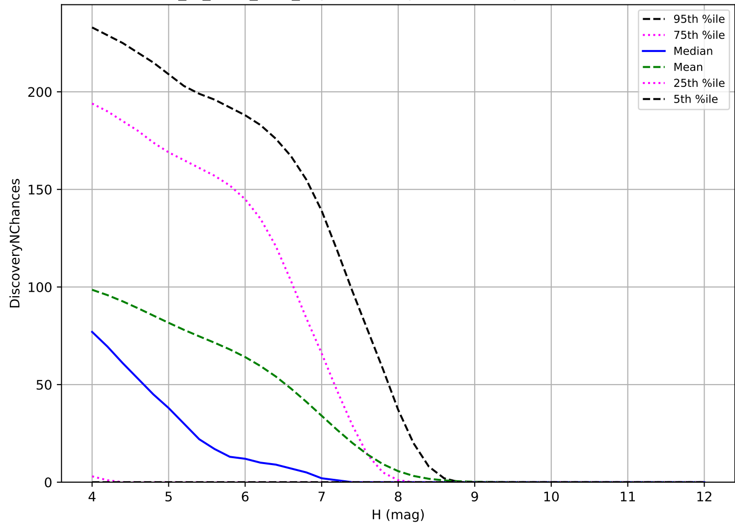
extra_ss_neo3_v3.4_10yrs: TNO 3 pairs in 15 nights detection loss
