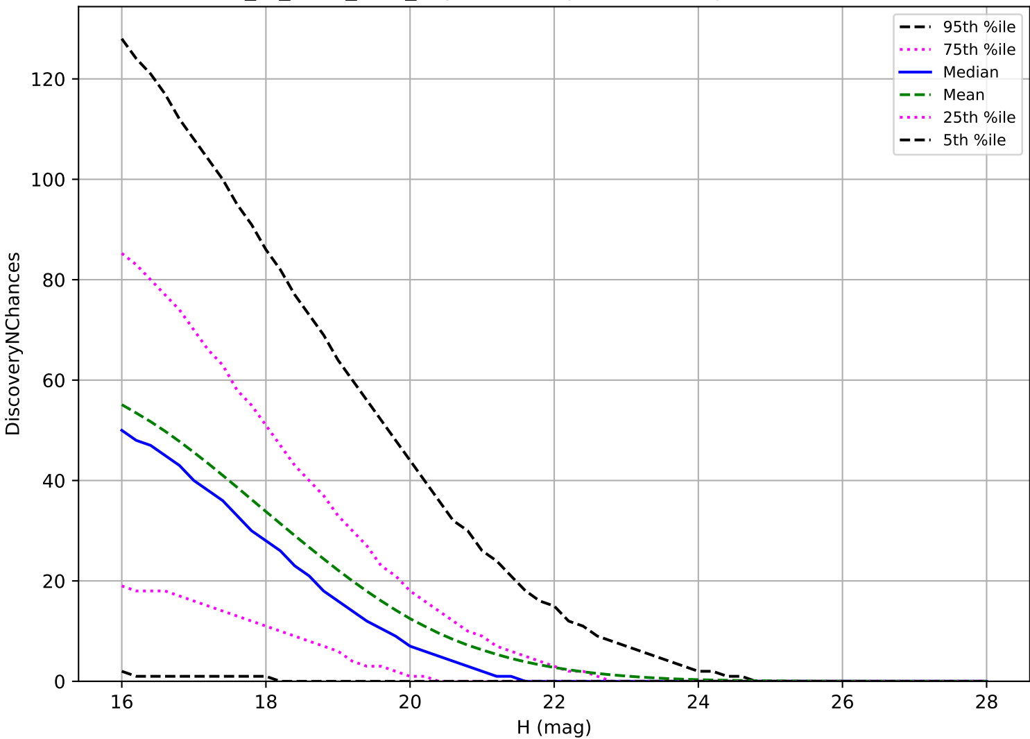
extra_ss_neo3_v3.4_10yrs: PHA 3 pairs in 15 nights detection loss
