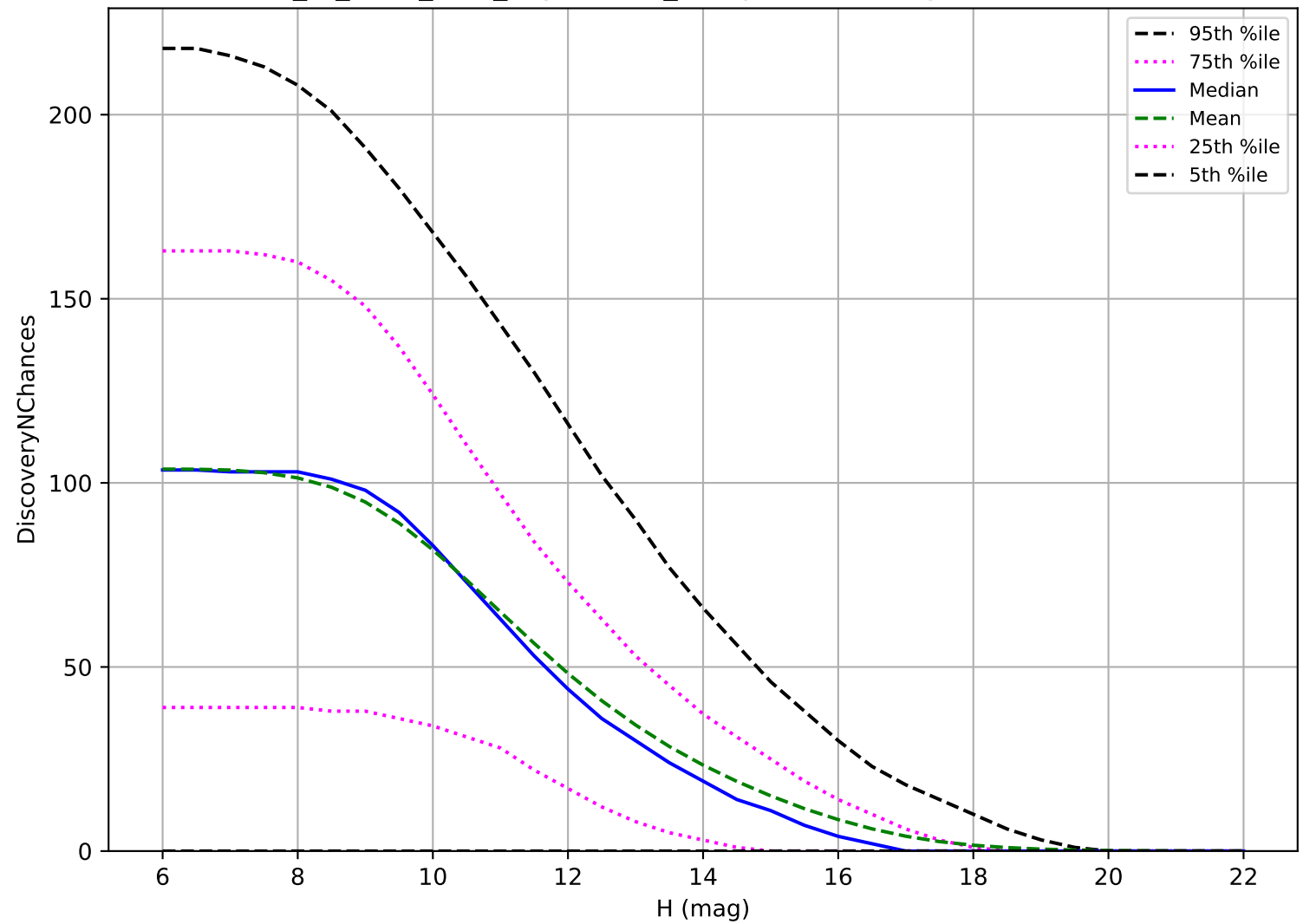
extra_ss_neo3_v3.4_10yrs: OCC_r5 3 pairs in 15 nights detection loss
