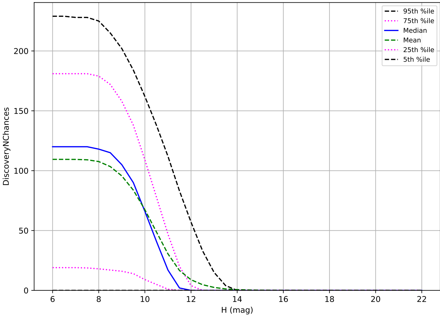
extra_ss_neo3_v3.4_10yrs: OCC_r20 3 pairs in 15 nights detection loss
