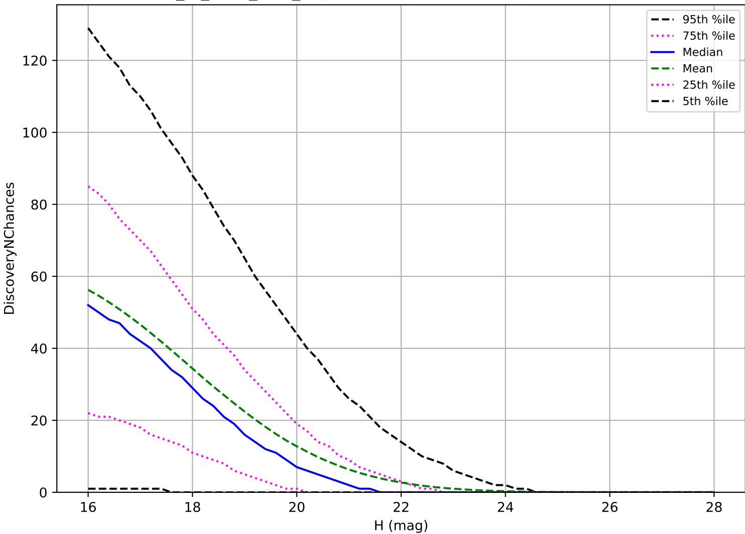
extra_ss_neo3_v3.4_10yrs: NEO 3 pairs in 15 nights detection loss
