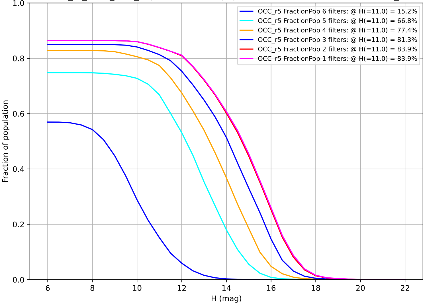
extra_ss_neo3_v3.4_10yrs: Fraction of population with colors in X filters OCC_r5
