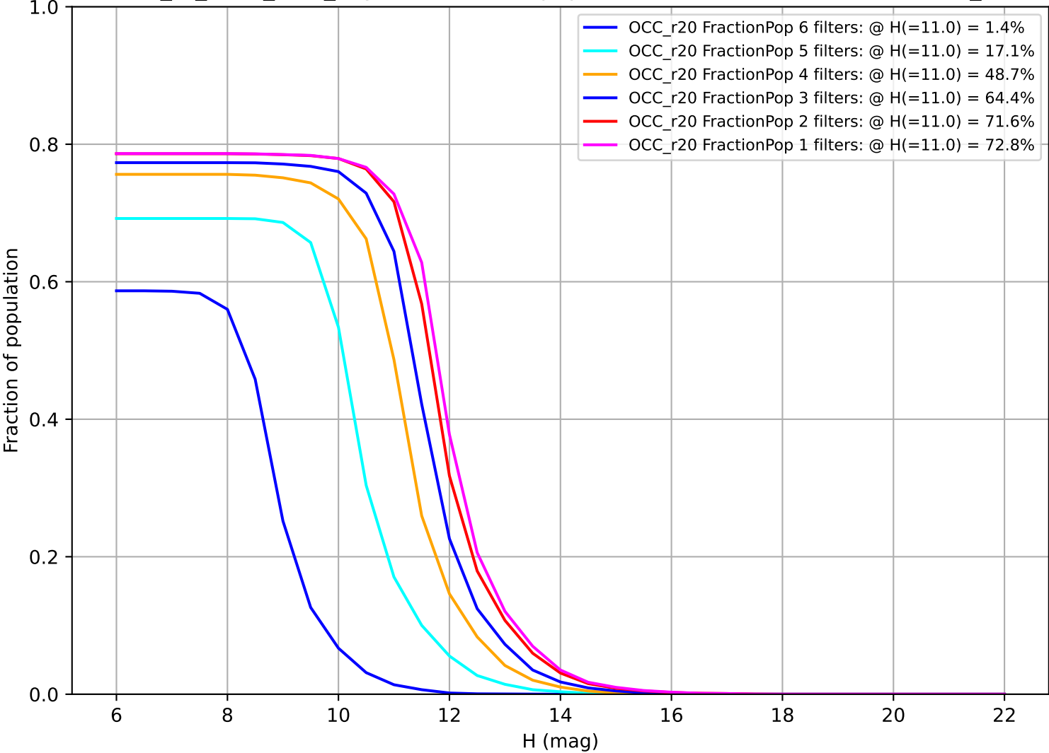
extra_ss_neo3_v3.4_10yrs: Fraction of population with colors in X filters OCC_r20
