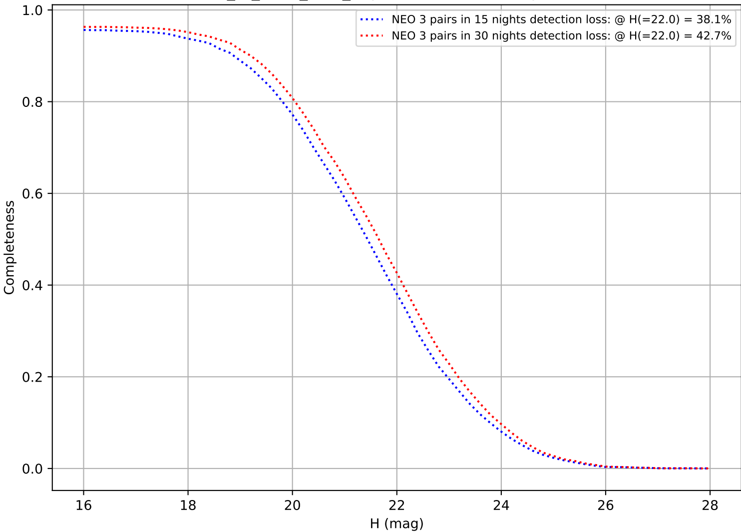
extra_ss_neo3_v3.4_10yrs: DifferentialCompleteness
