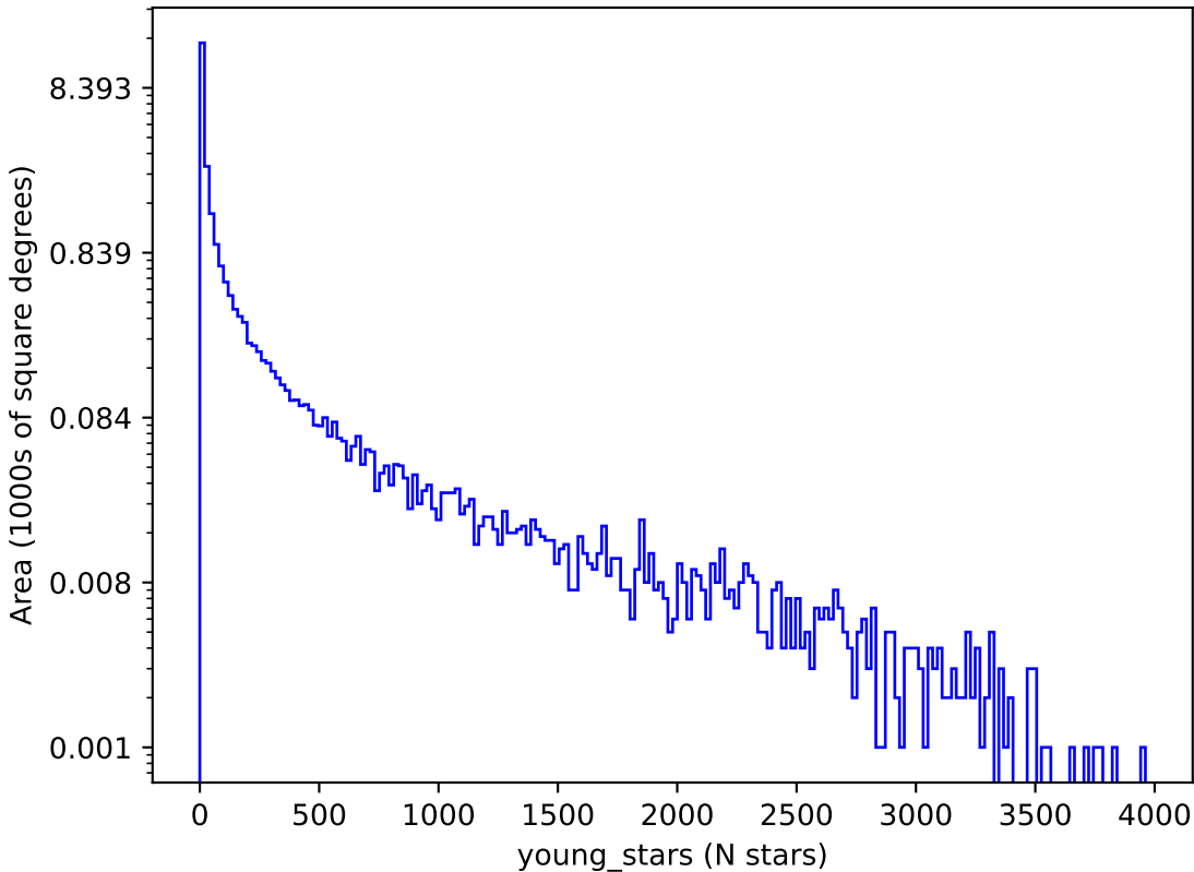
extra_ss_neo3_v3.4_10yrs : young_stars
