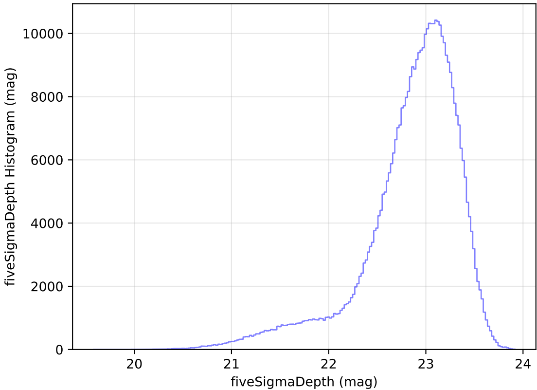
extra_ss_neo3_v3.4_10yrs z: fiveSigmaDepth Histogram
