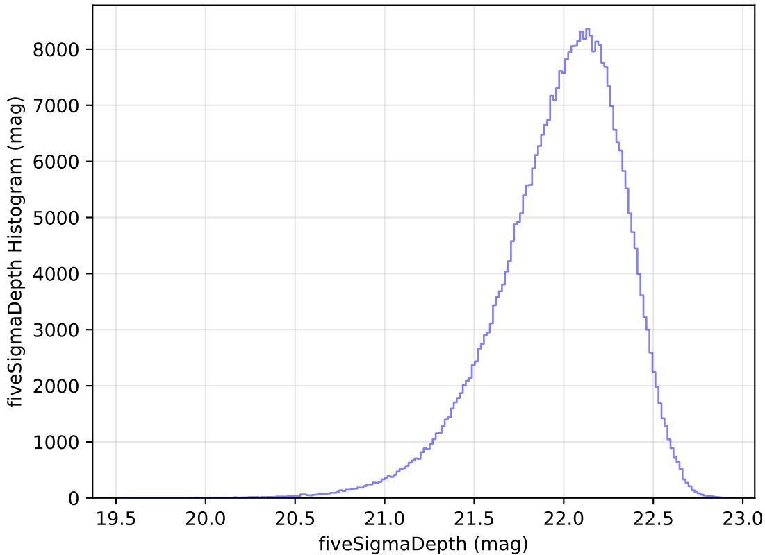
extra_ss_neo3_v3.4_10yrs y: fiveSigmaDepth Histogram
