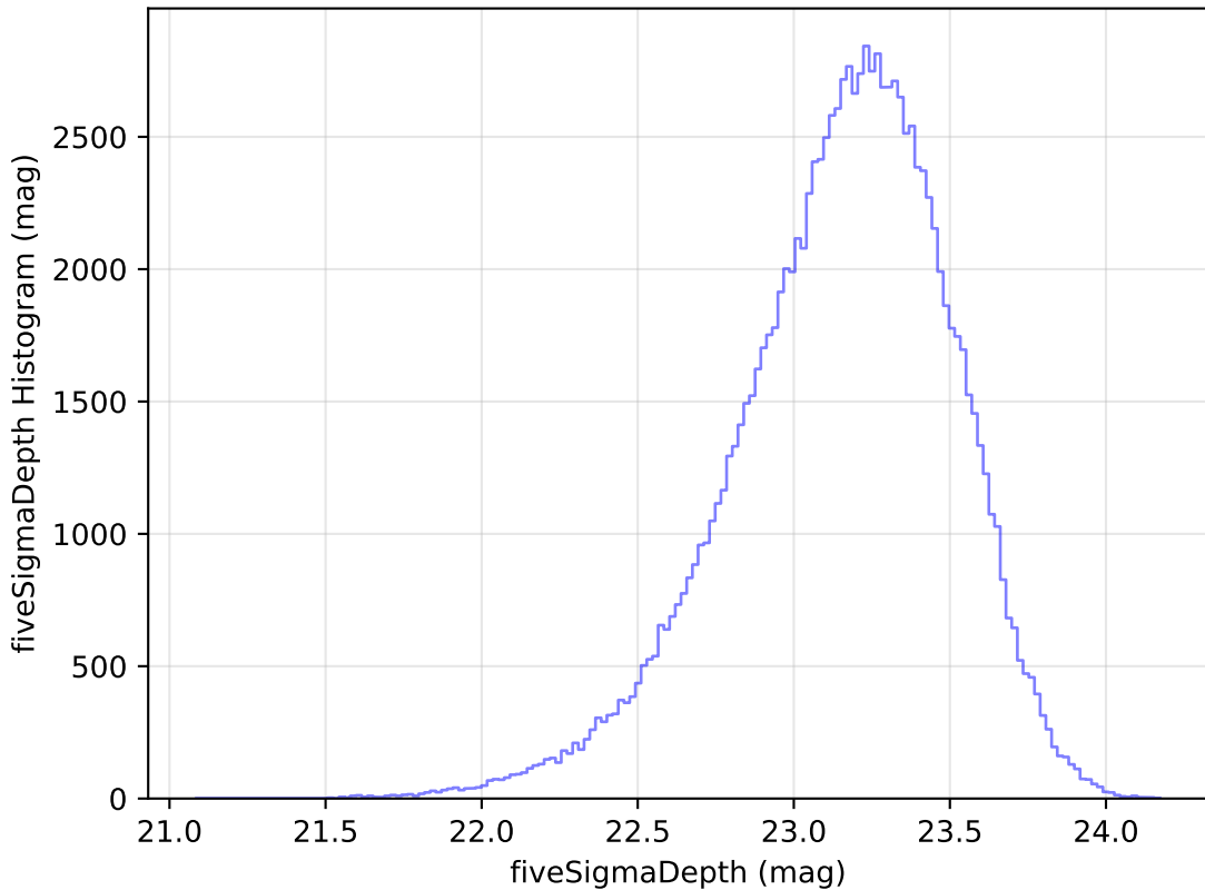
extra_ss_neo3_v3.4_10yrs u: fiveSigmaDepth Histogram
