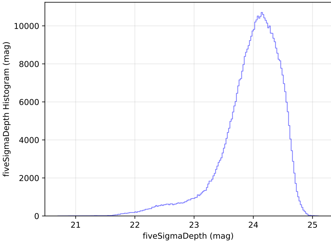
extra_ss_neo3_v3.4_10yrs r: fiveSigmaDepth Histogram
