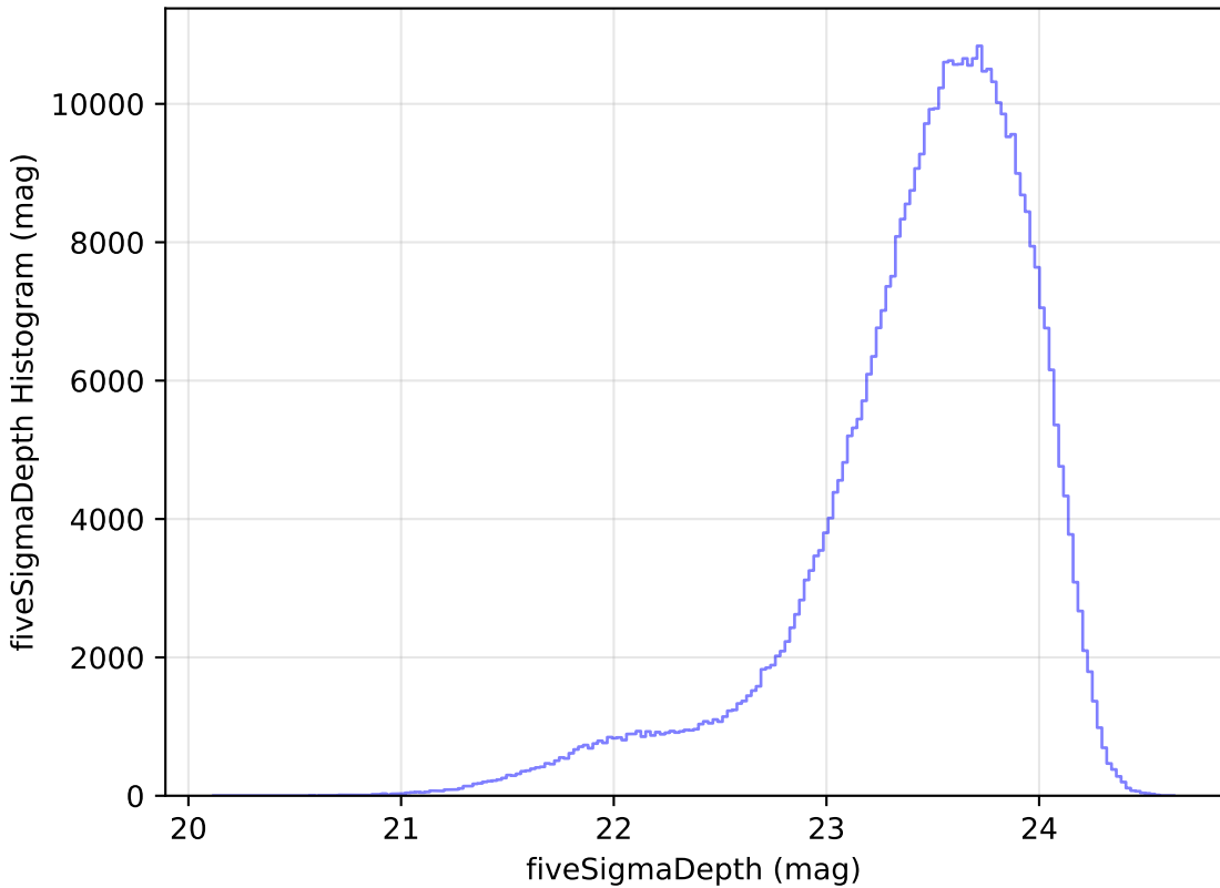
extra_ss_neo3_v3.4_10yrs i: fiveSigmaDepth Histogram
