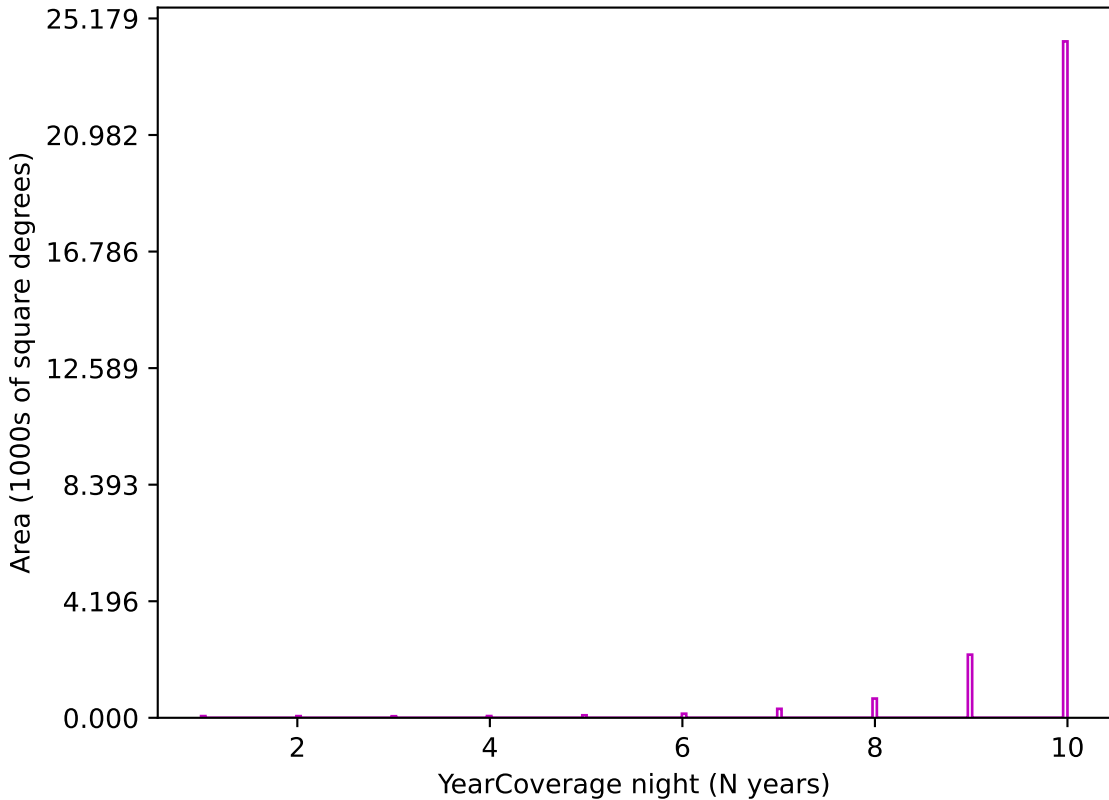
extra_ss_neo3_v3.4_10yrs z band: YearCoverage night
