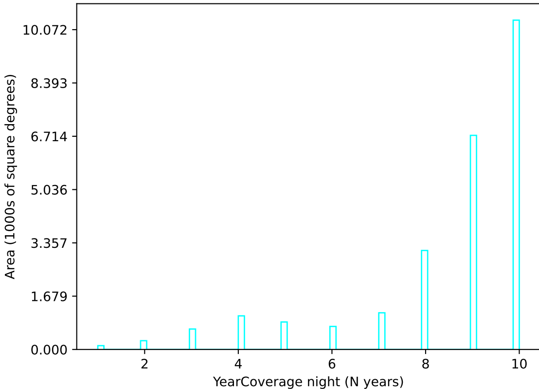
extra_ss_neo3_v3.4_10yrs u band: YearCoverage night
