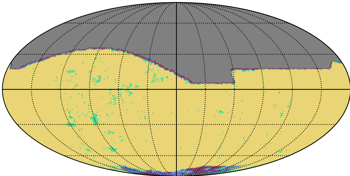
extra_ss_neo3_v3.4_10yrs r band: YearCoverage night
