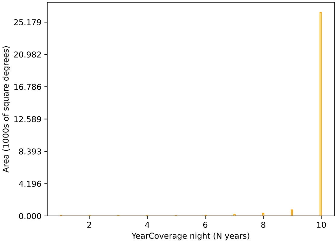
extra_ss_neo3_v3.4_10yrs r band: YearCoverage night
