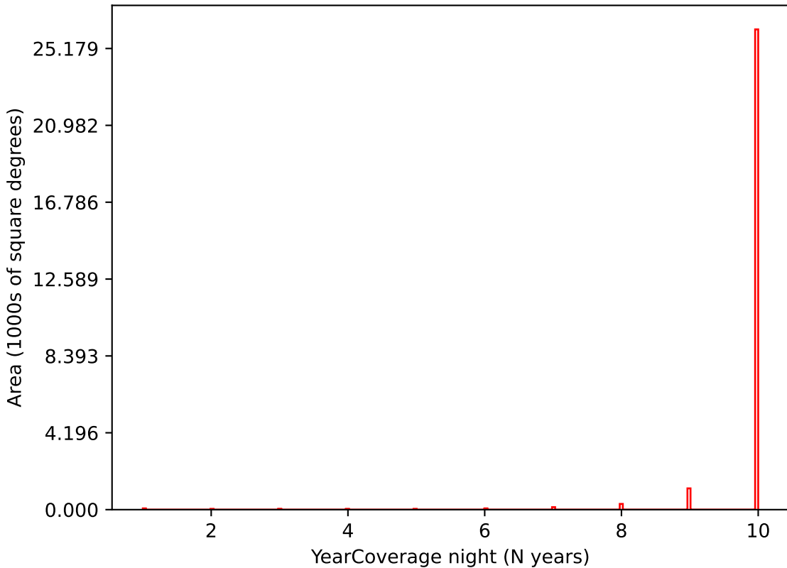
extra_ss_neo3_v3.4_10yrs i band: YearCoverage night
