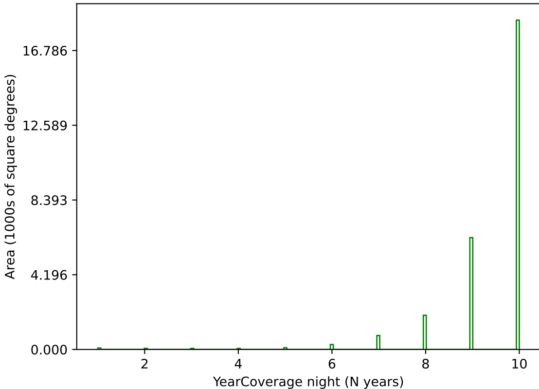
extra_ss_neo3_v3.4_10yrs g band: YearCoverage night
