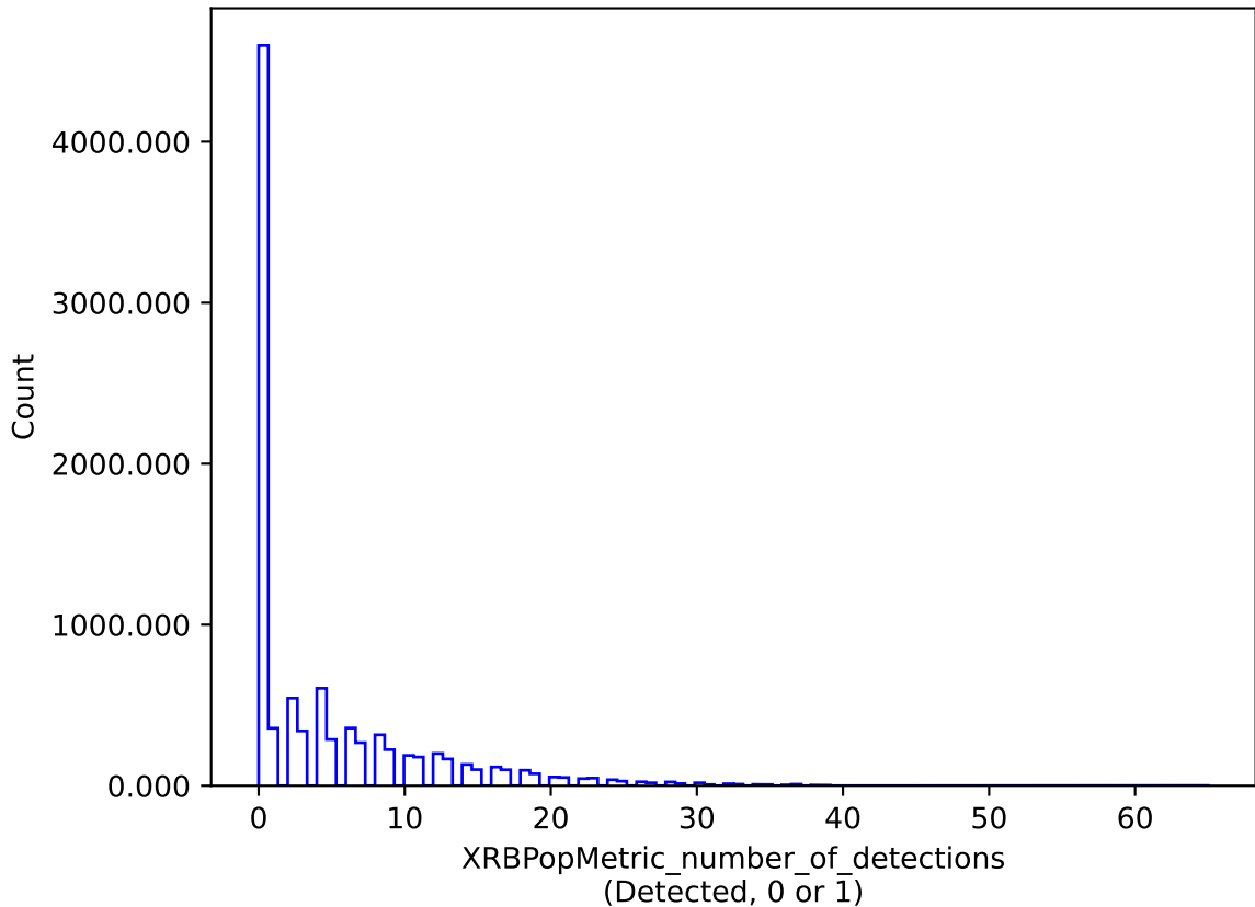
extra_ss_neo3_v3.4_10yrs : XRBPopMetric_number_of_detections
