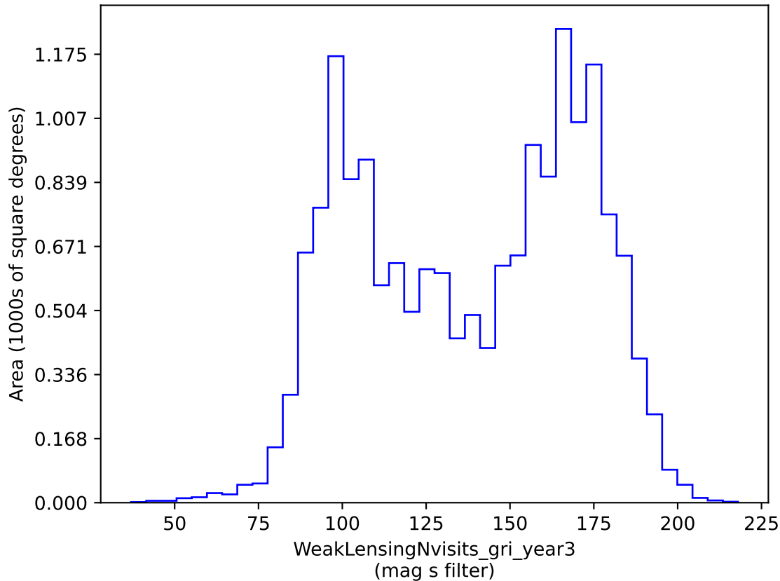
extra_ss_neo3_v3.4_10yrs gri band non-DD: WeakLensingNvisits_gri_year3
