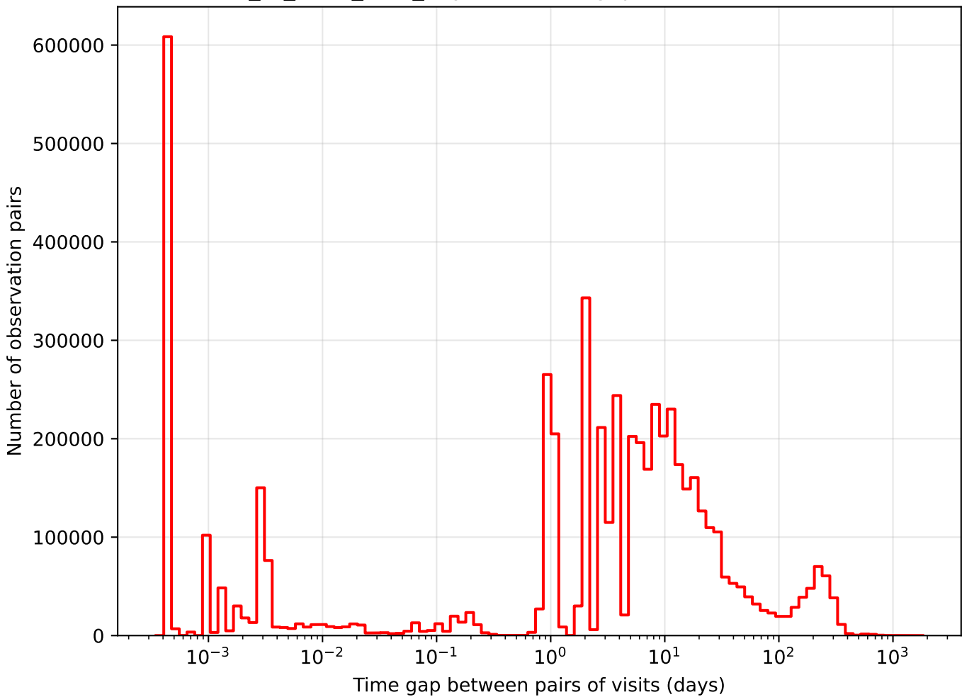
extra_ss_neo3_v3.4_10yrs i band: Tgaps observationStartMJD
