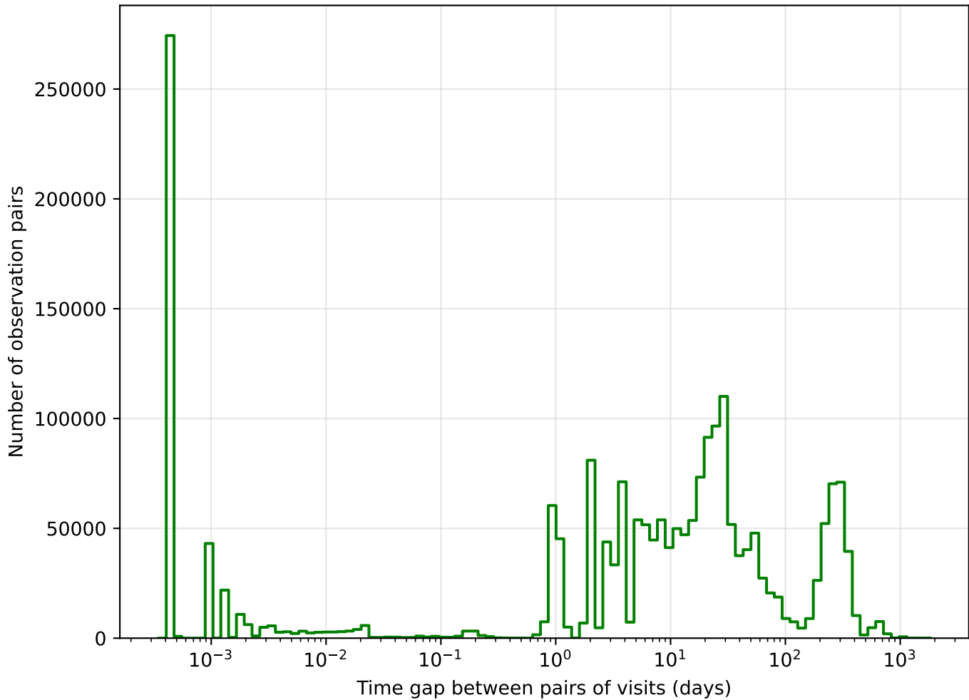
extra_ss_neo3_v3.4_10yrs g band: Tgaps observationStartMJD
