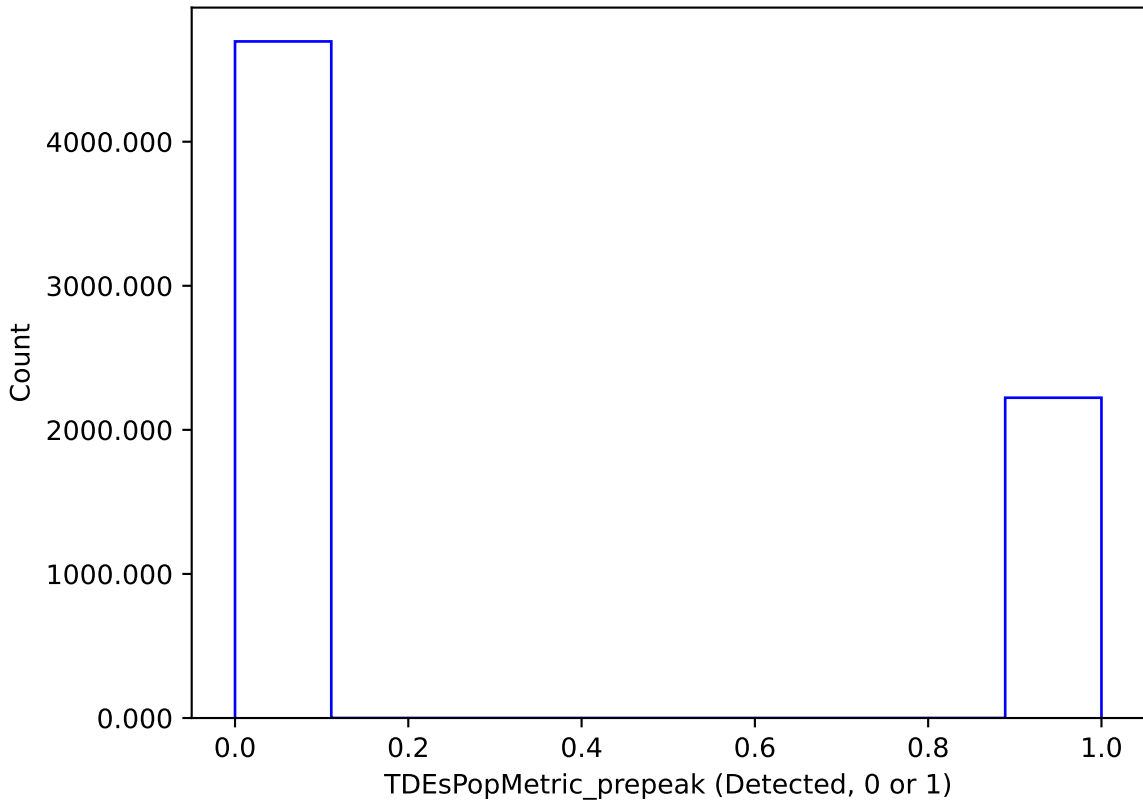
extra_ss_neo3_v3.4_10yrs : TDEsPopMetric_prepeak
