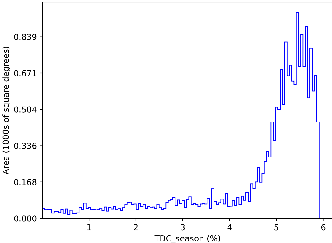
extra_ss_neo3_v3.4_10yrs : TDC_season
