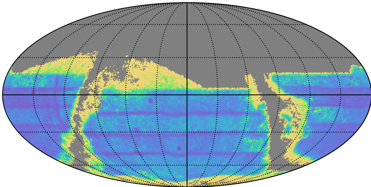
extra_ss_neo3_v3.4_10yrs : TDC_precision
