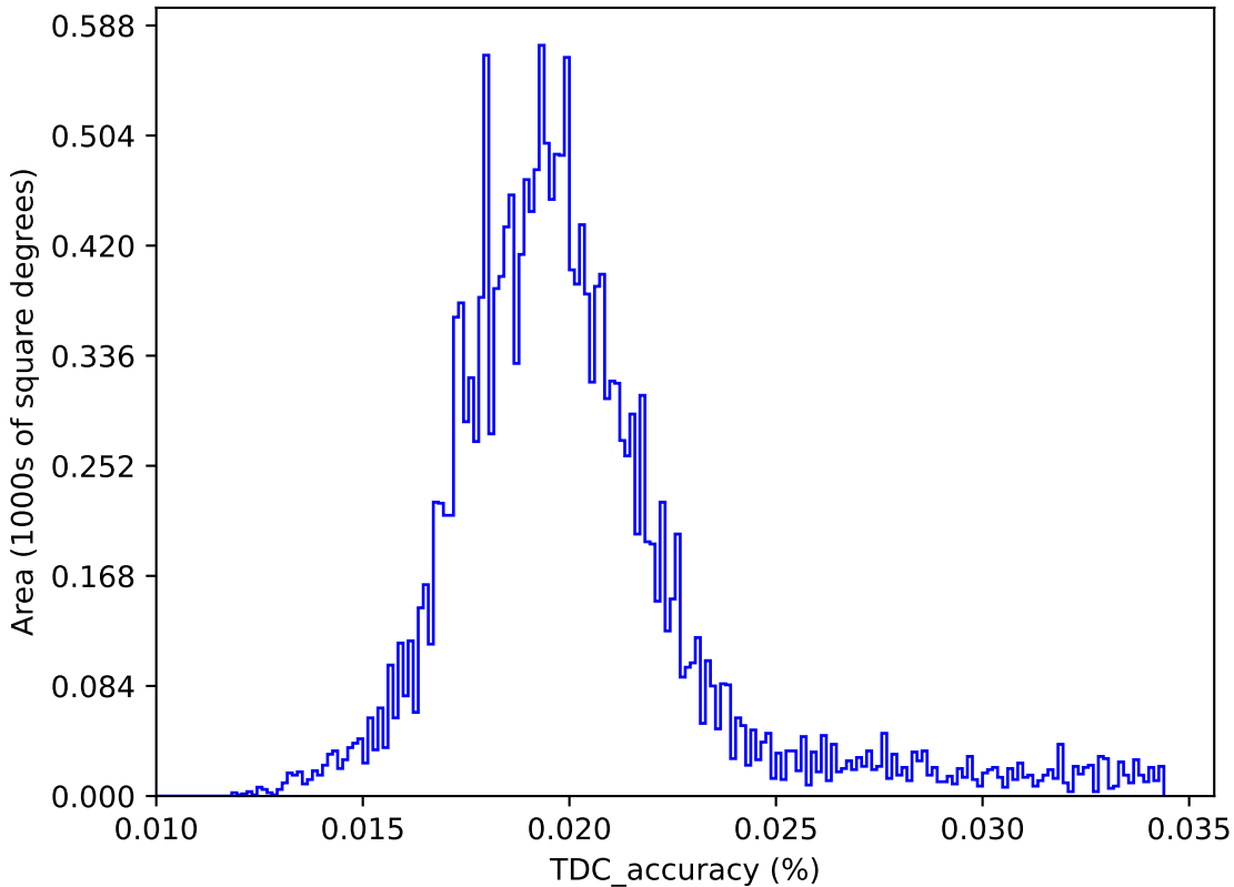
extra_ss_neo3_v3.4_10yrs : TDC_accuracy
