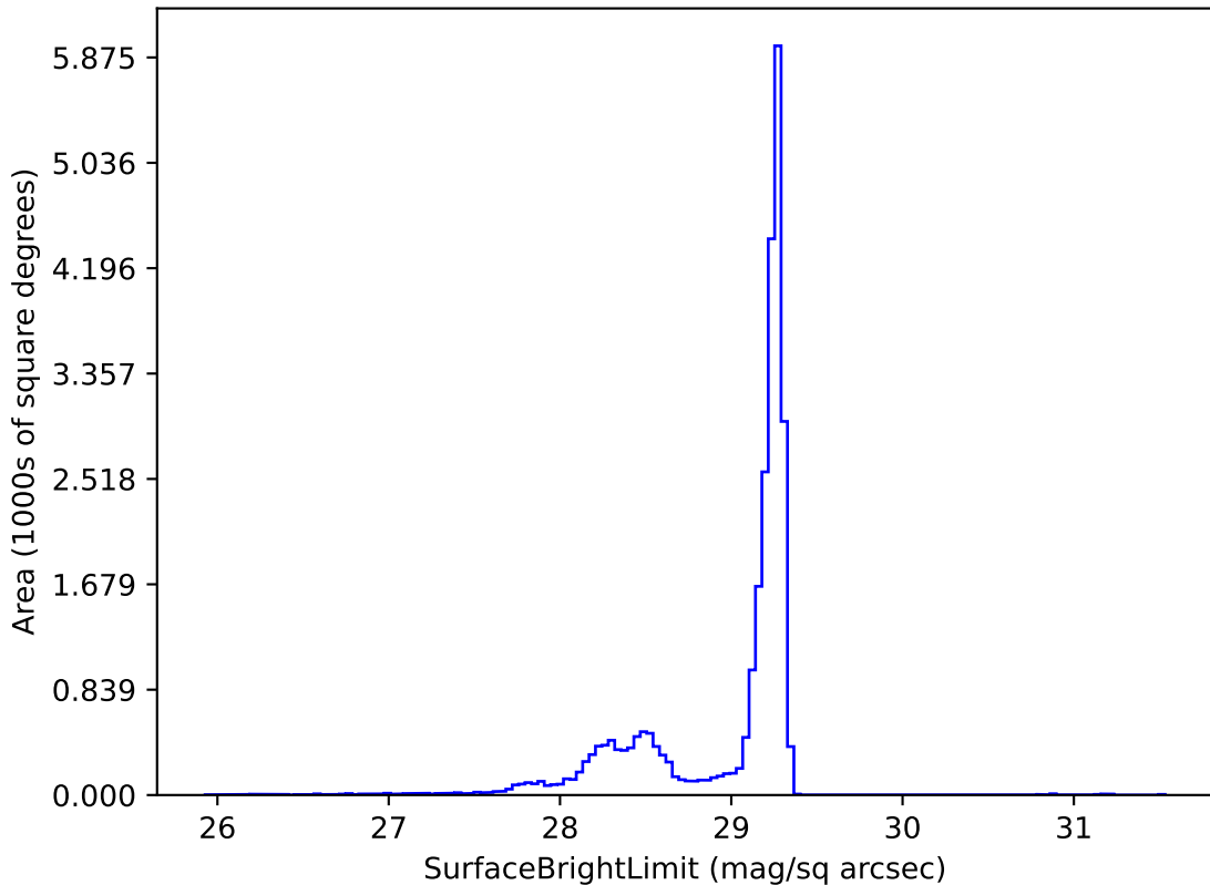
extra_ss_neo3_v3.4_10yrs z: SurfaceBrightLimit
