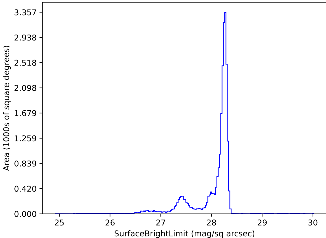
extra_ss_neo3_v3.4_10yrs y: SurfaceBrightLimit
