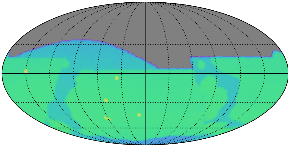
extra_ss_neo3_v3.4_10yrs r: SurfaceBrightLimit
