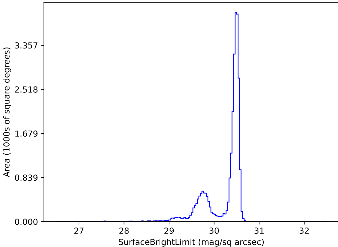
extra_ss_neo3_v3.4_10yrs r: SurfaceBrightLimit
