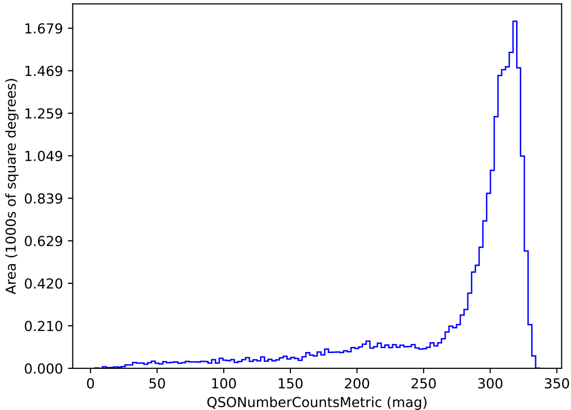
extra_ss_neo3_v3.4_10yrs u band and non-DD: QSONumberCountsMetric
