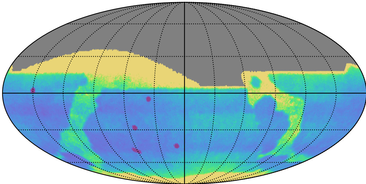
extra_ss_neo3_v3.4_10yrs : Proper Motion Uncert @ 24.0
