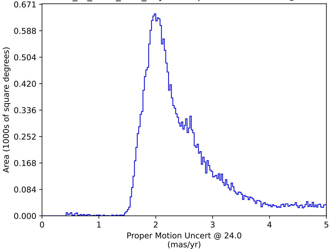
extra_ss_neo3_v3.4_10yrs : Proper Motion Uncert @ 24.0
