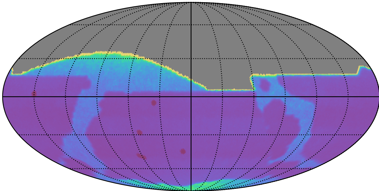
extra_ss_neo3_v3.4_10yrs : Proper Motion Uncert @ 20.5
