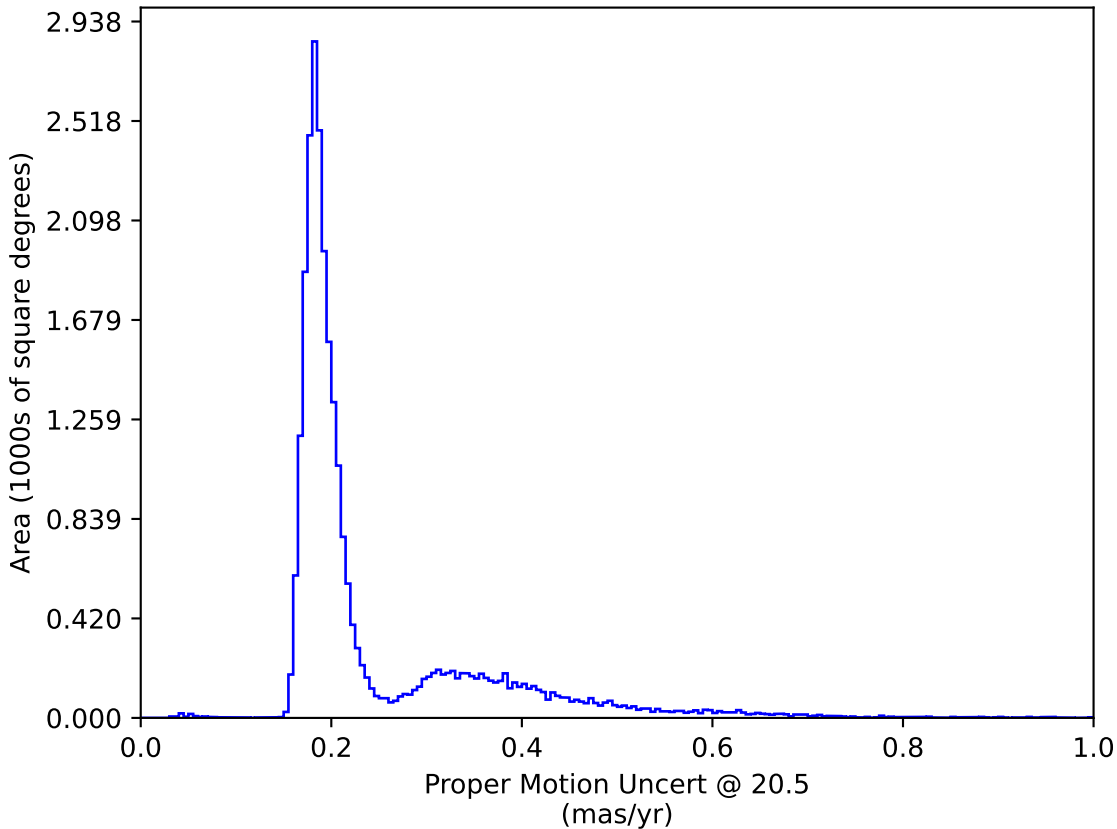
extra_ss_neo3_v3.4_10yrs : Proper Motion Uncert @ 20.5
