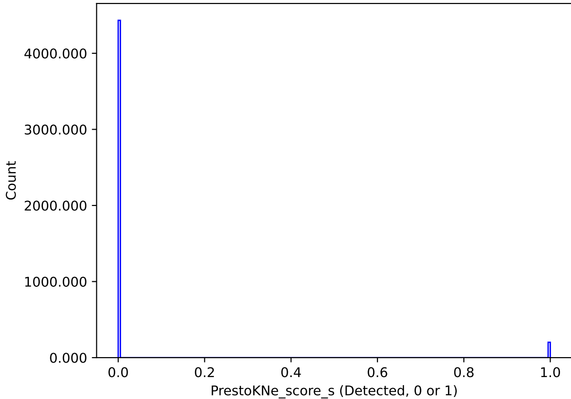
extra_ss_neo3_v3.4_10yrs : PrestoKNe_score_s
