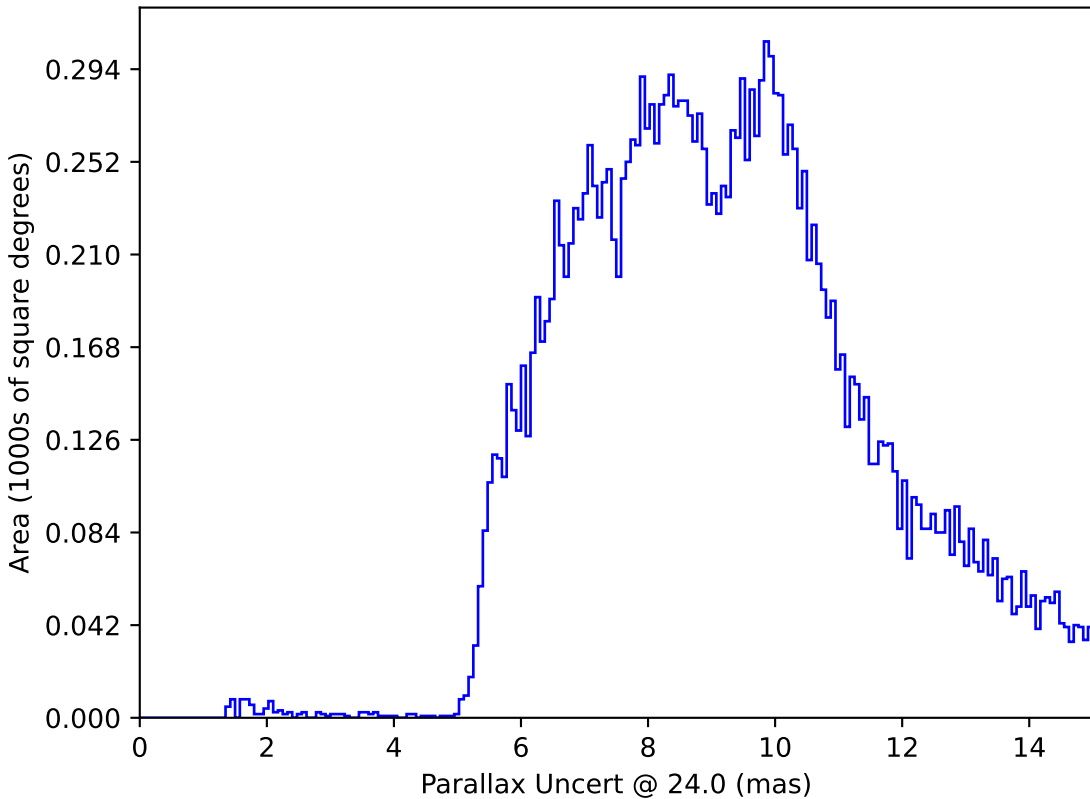
extra_ss_neo3_v3.4_10yrs : Parallax Uncert @ 24.0
