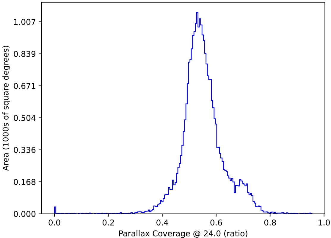
extra_ss_neo3_v3.4_10yrs : Parallax Coverage @ 24.0
