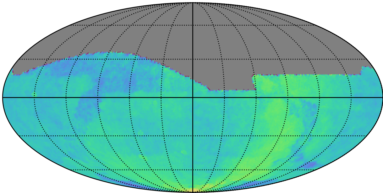
extra_ss_neo3_v3.4_10yrs : Parallax Coverage @ 22.4
