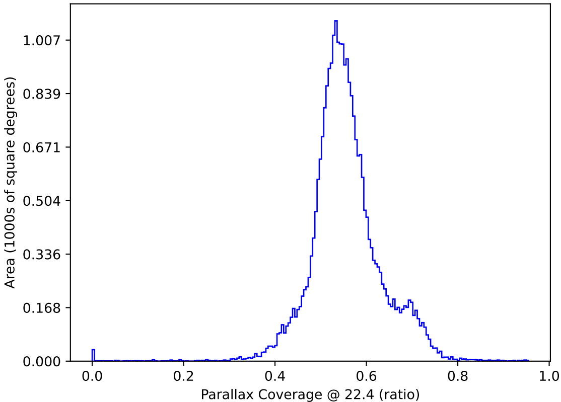
extra_ss_neo3_v3.4_10yrs : Parallax Coverage @ 22.4
