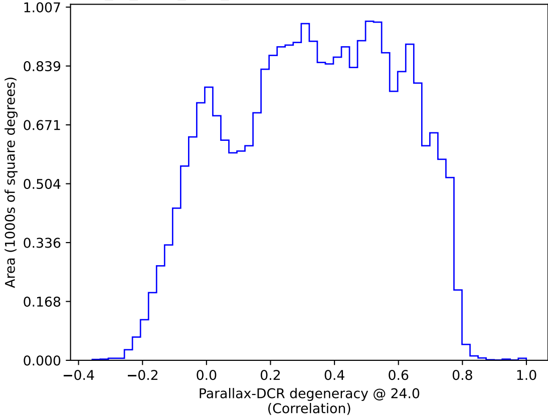
extra_ss_neo3_v3.4_10yrs : Parallax-DCR degeneracy @ 24.0
