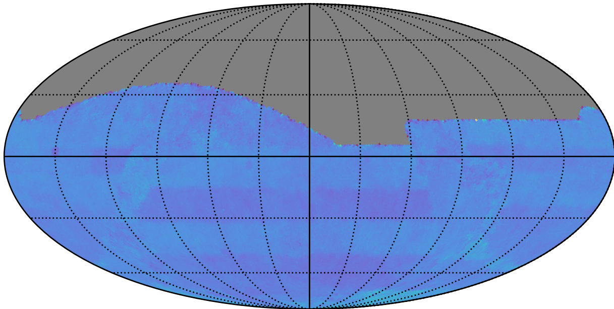
extra_ss_neo3_v3.4_10yrs : Normalized Proper Motion Uncert @ 24.0
