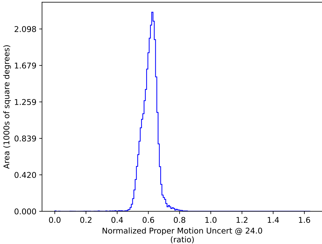
extra_ss_neo3_v3.4_10yrs : Normalized Proper Motion Uncert @ 24.0
