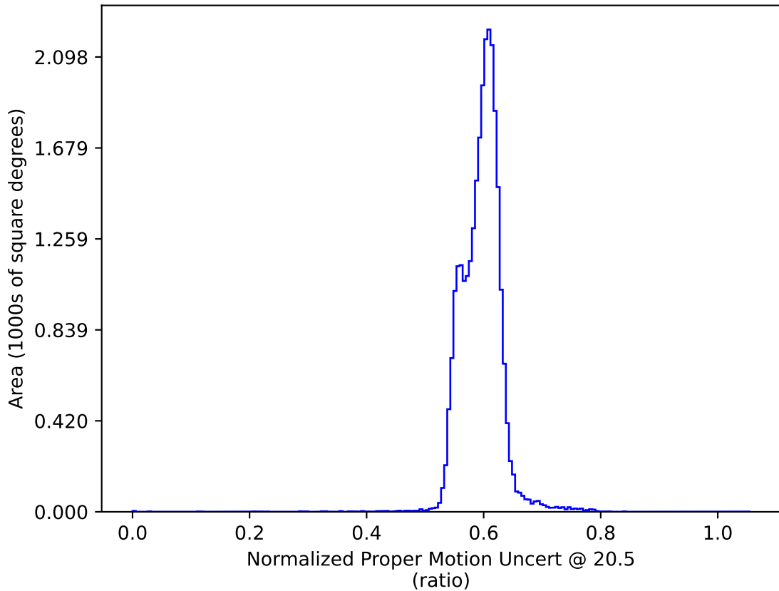
extra_ss_neo3_v3.4_10yrs : Normalized Proper Motion Uncert @ 20.5
