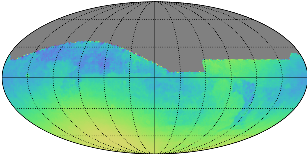
extra_ss_neo3_v3.4_10yrs : Normalized Parallax Uncert @ 24.0
